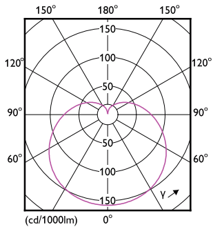
Light Distribution Diagram - LEDBulb 10.5-75W E27 2700K D 1PF/6 AU
