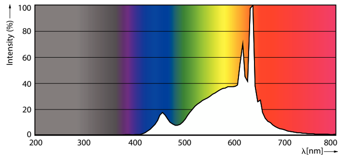
Spectral Power Distribution Colour - LEDBulb 10.5-75W E27 2700K D 1PF/6 AU
