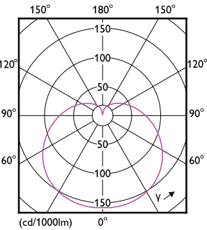
Light Distribution Diagram - LEDBulb 8.5-60W B22 2700K D 1PF/6 AU
