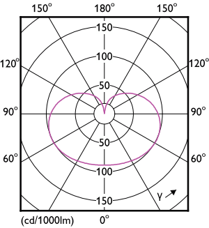
Light Distribution Diagram - LED Sensor 8-60W E27 CDL FR 1PF/6 APR
