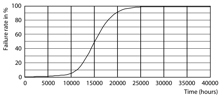
Life Expectancy Diagram - 4A19/PER/YELLOW/G/E26/ND 4/1PF
