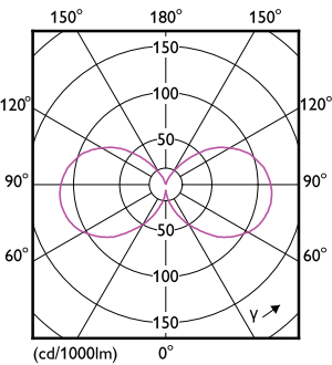
Light Distribution Diagram - 4A19/PER/RED/G/E26/ND 4/1PF
