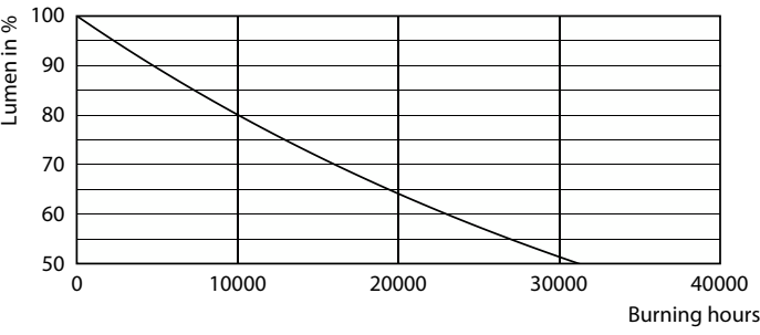
Lumen Maintenance Diagram - 4A19/PER/RED/G/E26/ND 4/1PF
