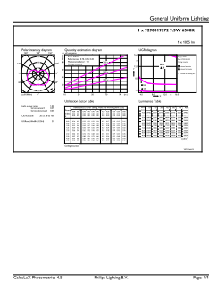
General uniform lighting - LEDStick 9.5W B22 6500K 1PF/6 AU
