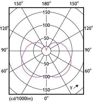
Light Distribution Diagram - LEDStick 9.5W B22 6500K 1PF/6 AU
