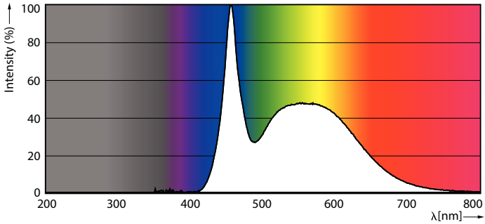
Spectral Power Distribution Colour - LEDStick 9.5W B22 6500K 1PF/6 AU
