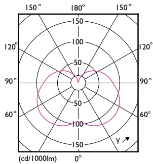
Light Distribution Diagram - CorePro LED Stick 7.5-57W E27 3CT 830
