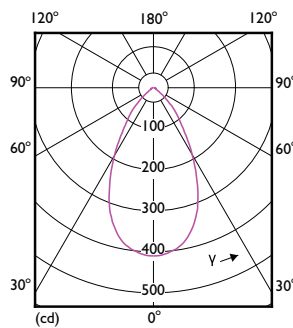
Light Distribution Diagram - LEDClassic 5-50W MR16 840 60D 6pack
