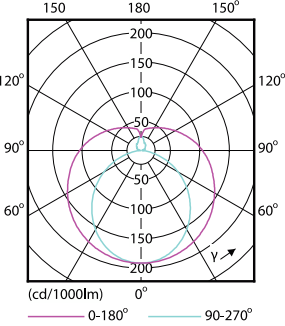
Light Distribution Diagram - LEDtube 1200mm 16W 765 T8 AP I G
