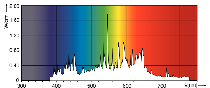
Spectral Power Distribution Colour - MASTERCoulour CDM-E MW eco 230W/842 E40
