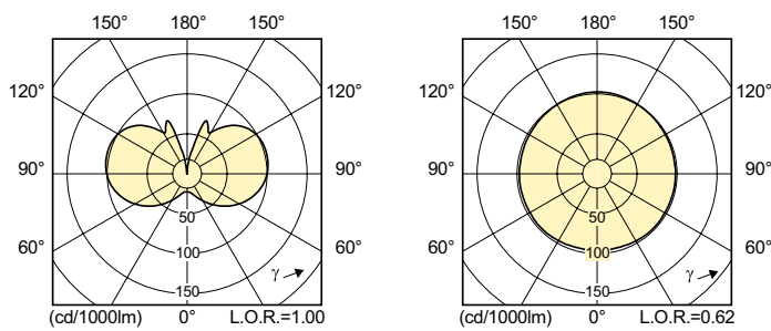
Light Distribution Diagram - MASTERCoulour CDM-E MW eco 230W/842 E40
