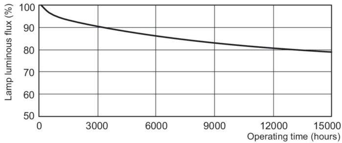
Lumen Maintenance Diagram - MASTER PL-S 11W/840/4P 1CT/5X10BOX
