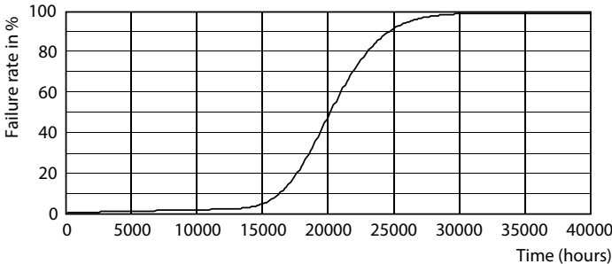
Life Expectancy Diagram - DN020B G3 LED9/CW 10.5W 220-240V D125SNI
