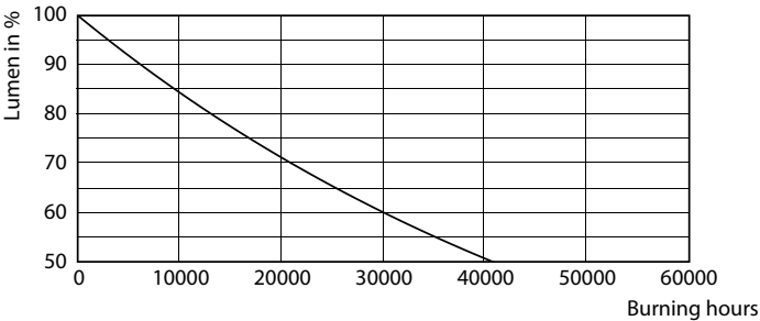
Lumen Maintenance Diagram - DN020B G3 LED9/CW 10.5W 220-240V D125SNI
