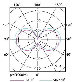
Light Distribution Diagram - CLA LEDCandle D 4.5-40W B35 E14 827 CL
