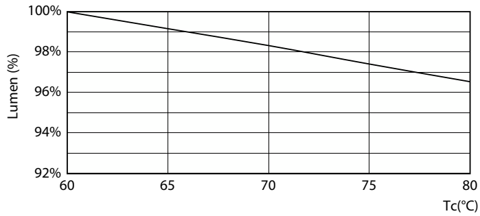
Lumen Maintenance Diagram - MAS LEDtube VLE UN 1500mm UO 24W865 T8
