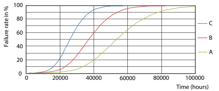
Life Expectancy Diagram - MAS LEDtube VLE UN 1500mm UO 24W840 T8
