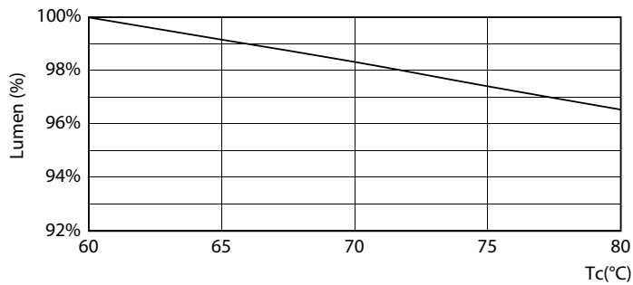
Lumen Maintenance Diagram - MAS LEDtube VLE UN 1500mm UO 24W840 T8
