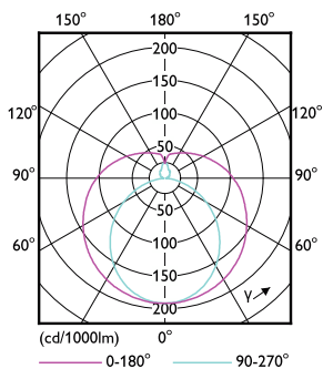
Light Distribution Diagram - MAS LEDtube VLE UN 1500mm UO 24W840 T8
