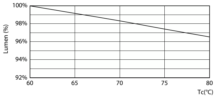
Lumen Maintenance Diagram - MAS LEDtube VLE UN 1200mm UO 16W840 T8
