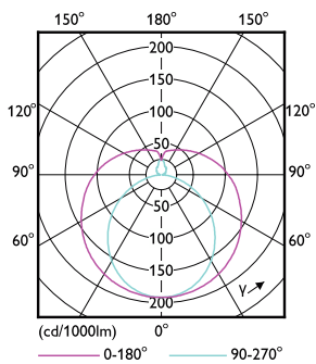
Light Distribution Diagram - MAS LEDtube VLE UN 1200mm UO 16W840 T8
