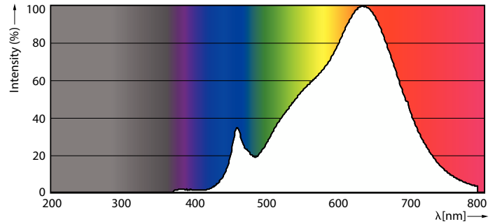
Spectral Power Distribution Colour - MAS LED ExpertColor 15-75W 927 AR111 40D
