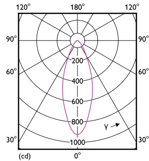
Light Distribution Diagram - 7PAR20/COR/827/F40/DIM/120V B 6/1FB
