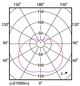
Light Distribution Diagram - 45HB/LED/840/ND FB 6/1
