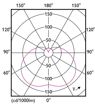
Light Distribution Diagram - 25HB/LED/850/ND FB 6/1
