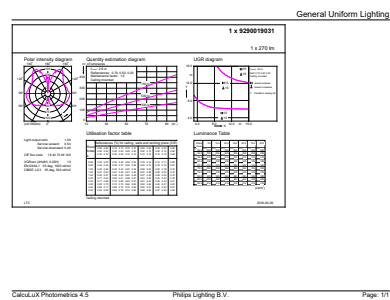
General uniform lighting - LED giant 25W E27 G200 4000K smoky D
