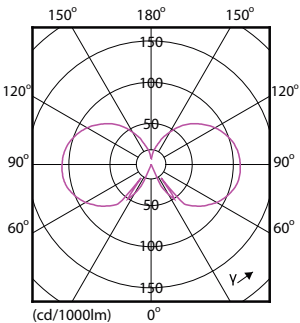
Light Distribution Diagram - CLA LEDLuster ND 2-25W P45 B22 827 CL
