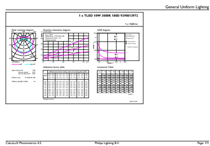
General uniform lighting - 10T8 LED/48-3000 IF 1PK 10/1
