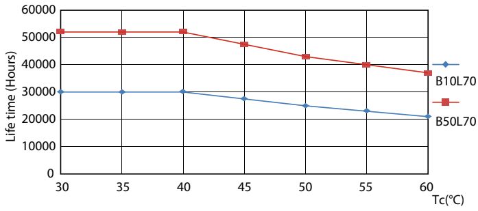
Life Expectancy Diagram - 10T8 LED/48-3000 IF 1PK 10/1
