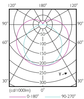
Light Distribution Diagram - 10T8 LED/48-3000 IF 1PK 10/1
