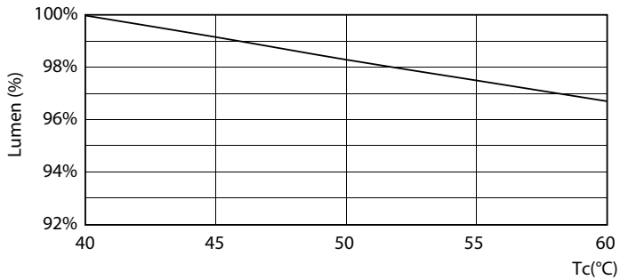
Lumen Maintenance Diagram - 10T8 LED/48-3000 IF 1PK 10/1
