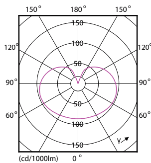
Light Distribution Diagram - LED SSW 100W A67 E27 WW-CW FR ND 1BC/6
