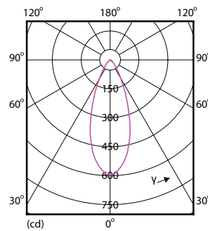
Light Distribution Diagram - 7PAR20/LED/F40/840/E26/GL/DIM 120V
