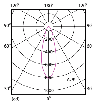
Light Distribution Diagram - 7PAR20/LED/F25/830/E26/GL/DIM 120V
