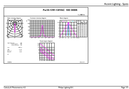
Accent Lighting Spots - 12PAR30S/EXPERTCOLOR RETAIL/S10/930/DIM
