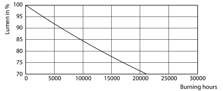
Lumen Maintenance Diagram - LED SSW 60W A60 E27 WW FR ND RF 1BC/6
