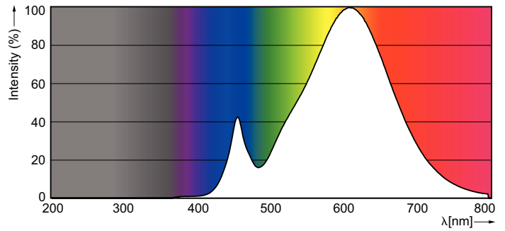
Spectral Power Distribution Colour - 6.5MR16/F35/2700-2200 DIM 12V
