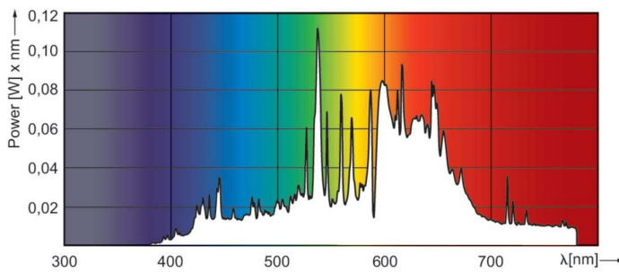
Spectral Power Distribution Colour - MASTERC CDM-R111 Elite 70W/930 GX8.5 40D
