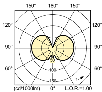
Light Distribution Diagram - MASTERC CDM-TC Elite 50W/942 G8.5 ICT
