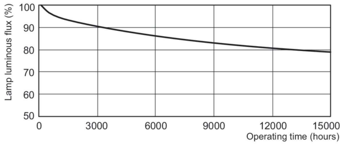
Lumen Maintenance Diagram - MASTER PL-S 11W/840/4P 1CT/5X10BOX
