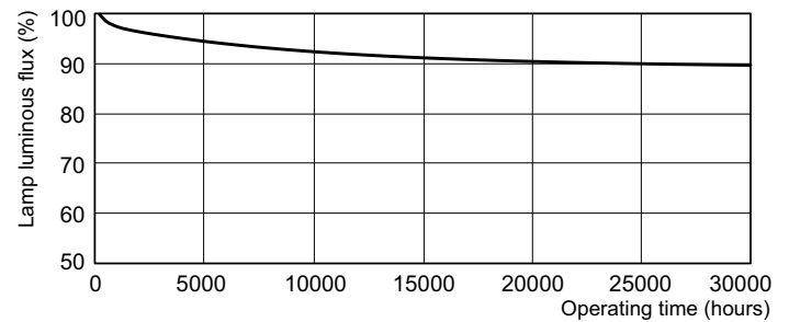
Lumen Maintenance Diagram - MASTER TL5 HO 54W/830 UNP/40
