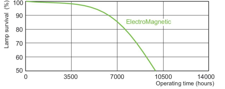
Life Expectancy Diagram - MASTER PL-C 13W/865/2P 1CT/5X10BOX
