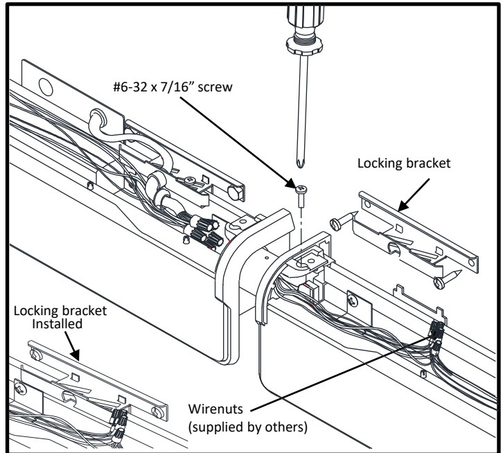
Secure fixture to straight joint with provided #6-32 x 7/16" screw. Install locking bracket, see step 11 for reference.
