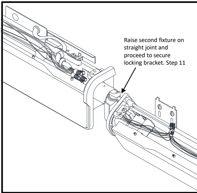
Raise fixture and feed wires through straight into second fixture.
