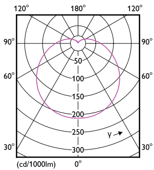
Light Distribution Diagram - LED 200W A110 E27 WW 230V FR ND 1PF/6
