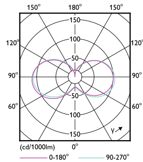
Light Distribution Diagram - TForce Core LED PT 30-27W E27 830 FR
